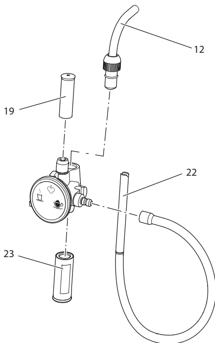
Abb. 16: Cappuccinatore zerlegen
